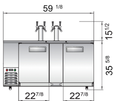
MCK-UDD-3-HC
