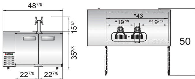
MCK-UDD-24-48SS-HC
