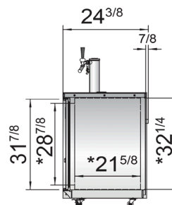
Side Dimensions
